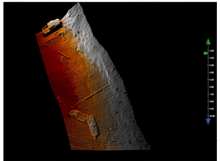
Figure 4: Single pass of sonar data showing the vehicle in question (top) and two other vehicles (bottom). Sonar image courtesy of SonarWiz.
